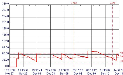
Typical VCS 1500 Level Readings displayed at dataqwestinc.com Web Site
